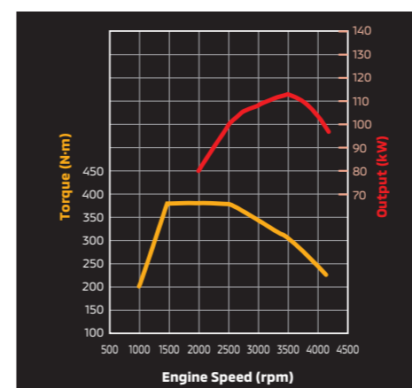
2.4-litre Turbocharged DOHC DI-D Standard (113kW/3500rpm, 380 N·m/1500-2500rpm)
